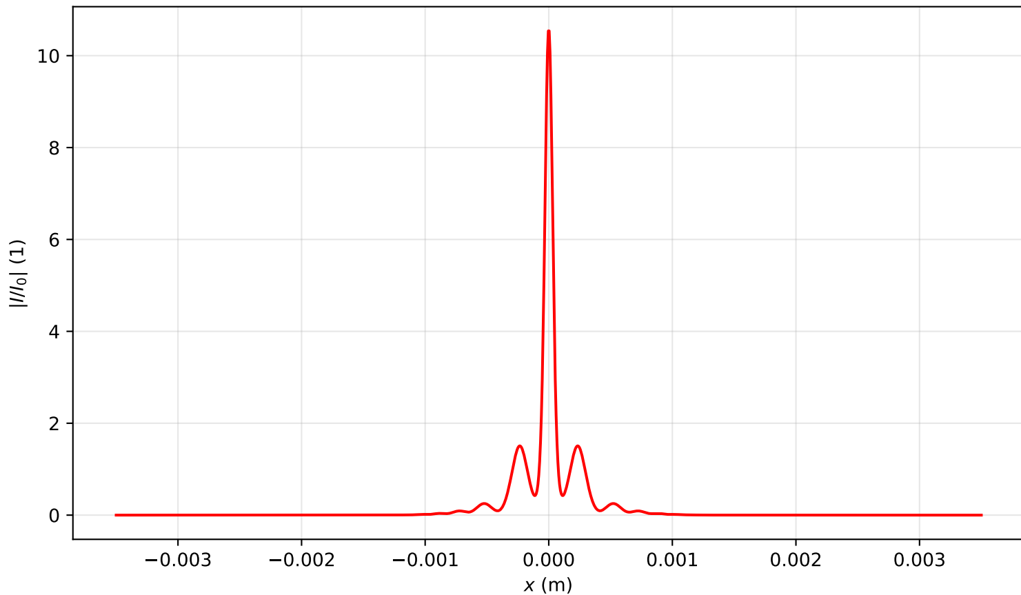
Intensity profile I(x, y = 0, z = 0.478)/I_0 , P_{in}=8.5P_{cr} , artificial time
